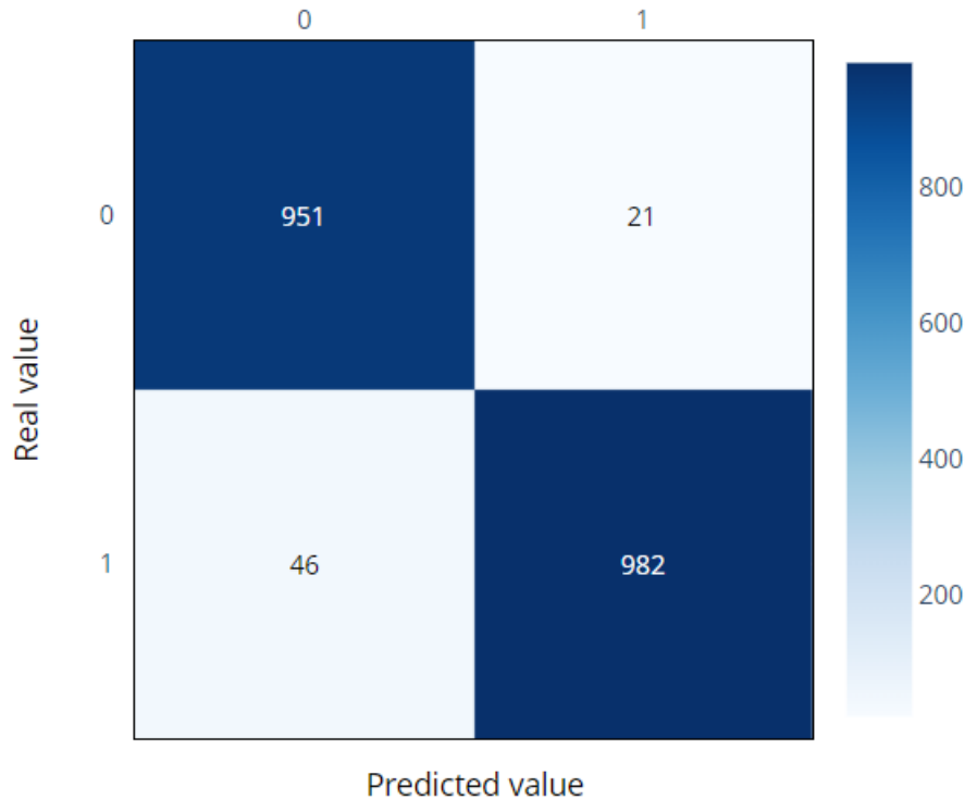
Confusion matrix
